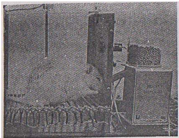
Fig 3.3 Skinner box
